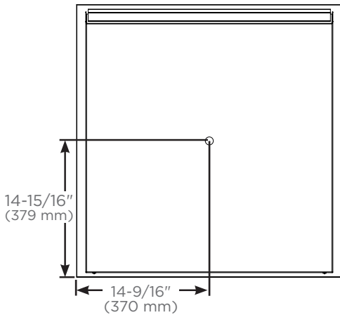
Back view for electrical knockout location
