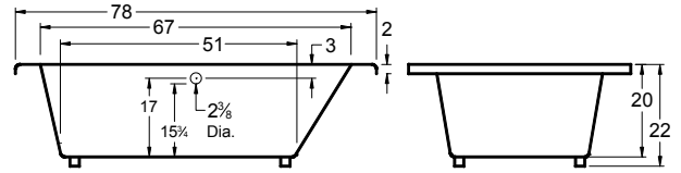
All bathtub dimensions are ± 1/2"
